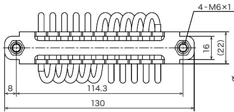
A type (安装部为螺丝)
